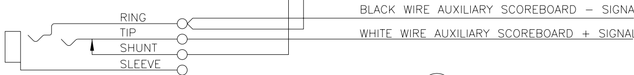
SCHEMATIC AUXILIARY 1/4" PHONE JACK
