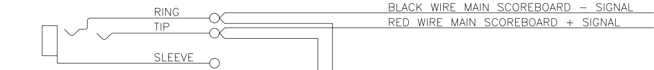
SCHEMATIC MAIN 1/4" PHONE JACK
