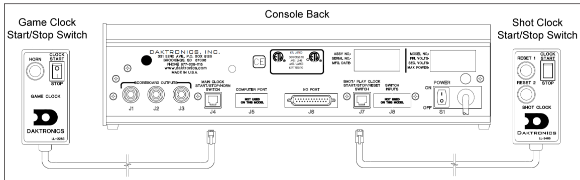
Figure 3: Remote Start/Stop Switches
