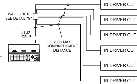
DETAIL "F"
